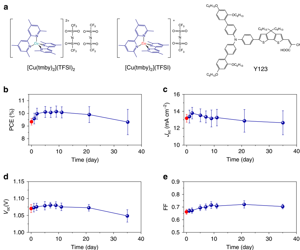
Figure 1 | DSCs with the Cu(II/I) hole conductor and Y123 sensitizer. (a) Schematic structures of the hole conductors based on [Cu(4,4',6,6'-tetramethyl-2,2'-bipyridine) 2 ](bis(trifluoromethylsulfonyl)imide) 2 ([Cu(tmby) 2 ](TFSI) 2 ) and [Cu(4,4',6,6'-tetramethyl-2,2'-bipyridine) 2 ](bis(trifluoromethylsulfonyl)imide), ([Cu(tmby) 2 ](TFSI)) and the dye molecule Y123. (b) Evolution of the PCE of unsealed DSCs. (c) Evolution of the J_{sc} of unsealed DSCs. (d) Evolution of the V_{oc} of unsealed DSCs. (e) Evolution of the FF of the unsealed DSCs. The unsealed DSCs were stored in ambient air in the dark. The photovoltaic parameters of solar cells were measured under standard AM1.5G conditions. The red symbols and error bars denote the sealed DSCs based on the volatile electrolyte. The royal blue symbols and error bars denote unsealed DSCs. The average (symbols) and s.d. (error bars) were calculated from solar cells numbering between 4 and 22.
